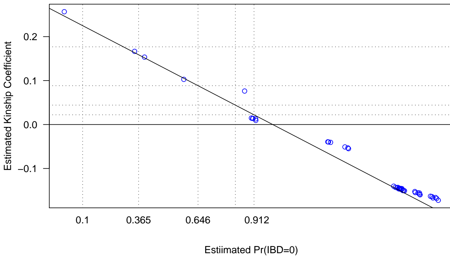
KING-Homo
